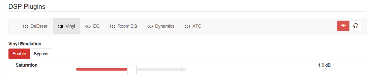
Figure 6: Vinyl plugin
