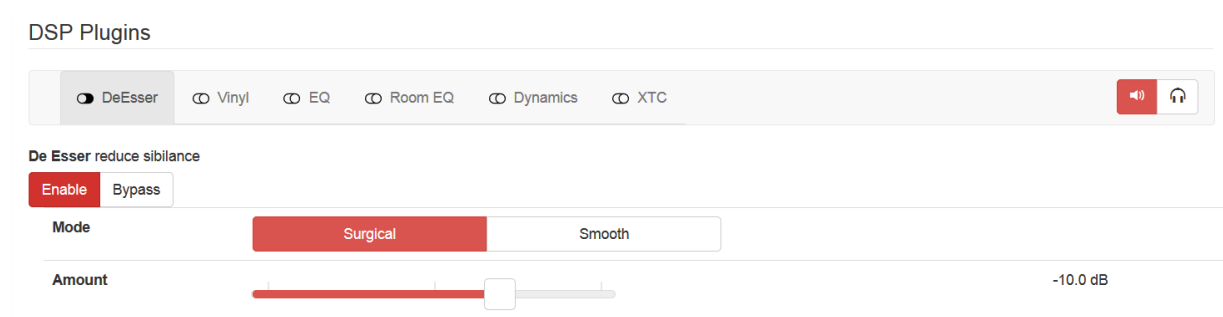
Figure 5: De-Esser plugin
